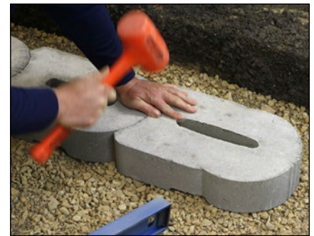
Diagram 19—Lay and level base block
